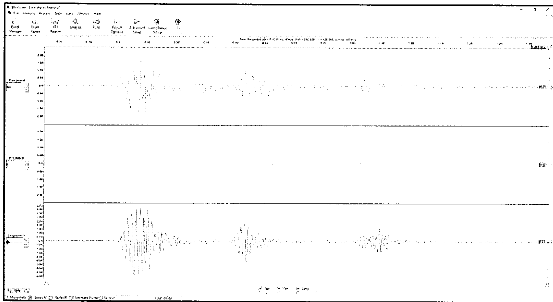
Figure 4. Blast time history recorded on 07.07.2024 at mine boundary near the house of Mr. Sultan Ahmad.
